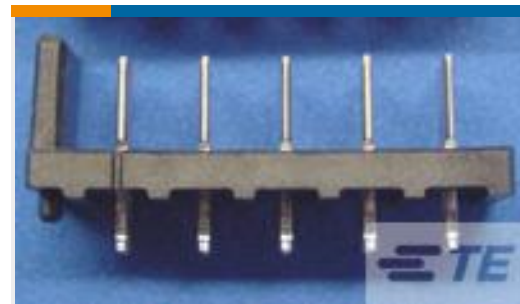
TE Part #5787419-1 HDR ASY, VERT, STR TAIL, 10.8V
