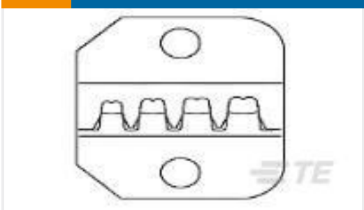
TE Part #90683-2 PROCRIMPER DIE ASSY DYNAMIC
