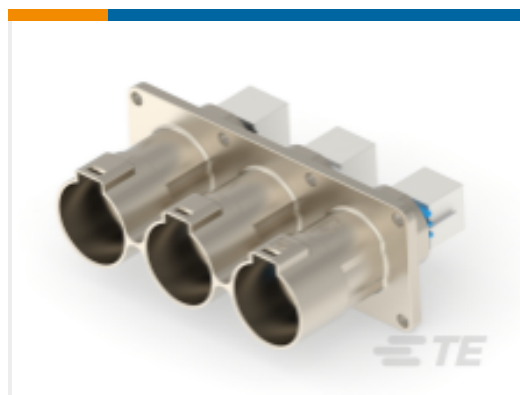
TE Part #2399608-1 3POS,HVP1400,ASSY,180DEG,COD A /B/C
