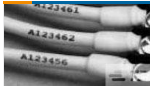
TE Part #5053164039 RNF-100-3/8-4-SP
