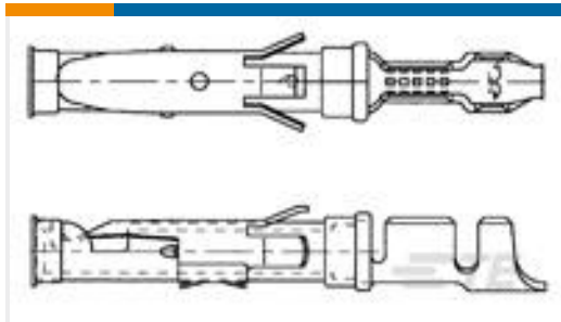
TE Part #1-163083-1 .062 DIA SOC.ASS 3+
