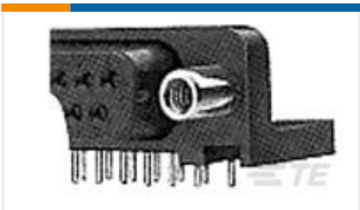
TE Part #5788799-1 15 HTMSFL ASSY RA 318 (SL,BL)
