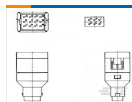
TE Part #65003-06N RECP ASSY
