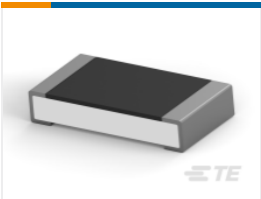
TE Part #5-2176388-5 RQ 1206 36R5 0.1% 10PPM 5K RL
