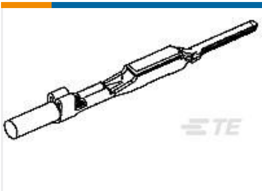
TE Part #316834-1 040-3 SEALED CONT TAB S
