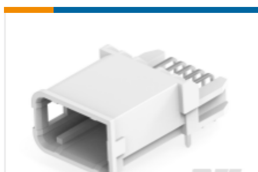
TE Part #2331207-2 10POS,TAB0.5X0.4,HDR ASSY,90DEG, COD B
