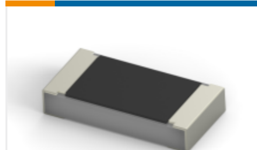
TE Part #4-1614958-0 CPF 0805 2R49 0.1% 25ppm 1K RL
