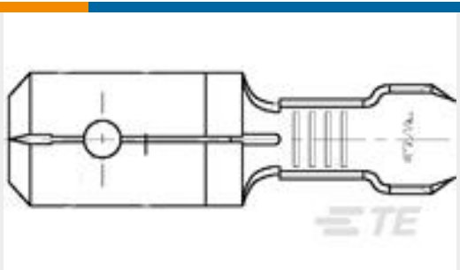
TE Part #42474-3 250 FASTON TAB 18-14 AWG BR
