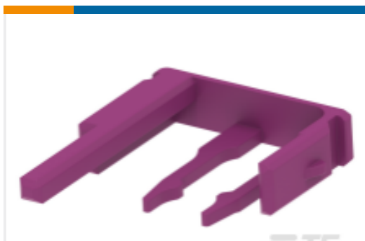
TE Part #1-2351080-1 57POS, HYBRID, REC HSG, SECONDARY LOCK
