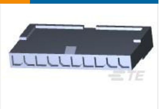
TE Part #1-1445049-0 FREE HANG SNGL ROW HSG 10 POS
