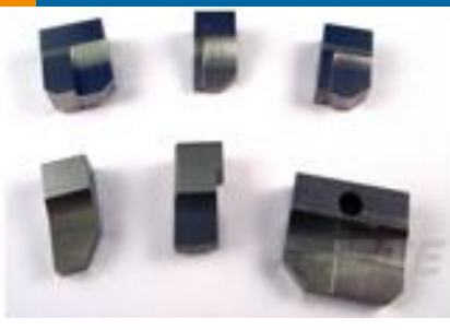
TE Part #2-690471-9 COMB ANVIL
