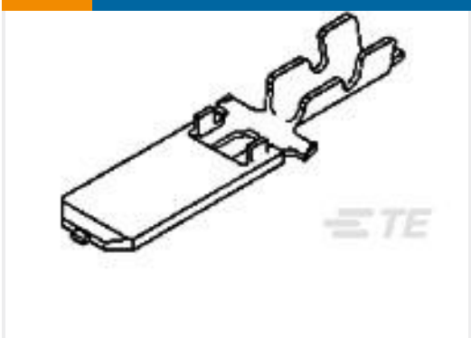
TE Part #170340-3 FF 250 TAB 20-14AWG PTBR WITHOUT LATCH
