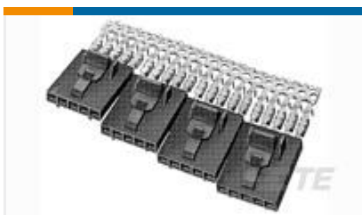
TE Part #5-103957-2 8X3 MTE RCPT SR LATCH .100CL
