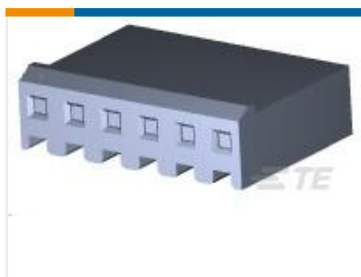
TE Part #640250-6 06P SL156 HSG W/LCK RAMP NATL
