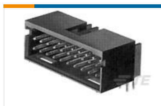
TE Part #6-102570-1 26 MODII HDR DRRA SHRD LF
