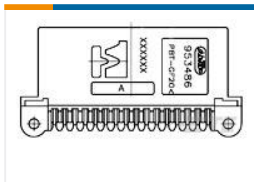
TE Part #953486-1 32pos MQS .63 header 90deg
