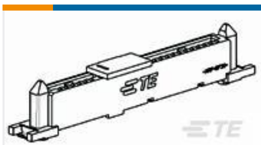
TE Part #1-1827864-0 Receptacle and Tab Housing: 2.5 mm Pitch, 250V
