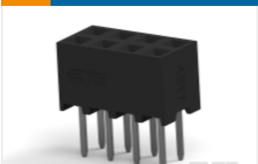
TE Part #2314822-8 8P,2MM,B-B,REC,DRVT,2.7,0.76AU,TB
