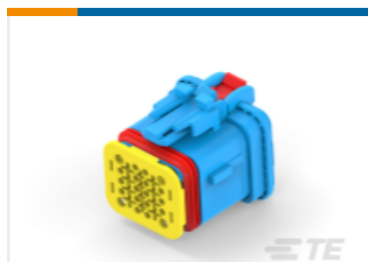
TE Part #2350890-4 20POS, HYBRID, SOC HSG ASSY, SLD, COD D
