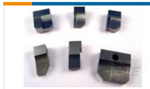
TE Part #1333207-2 ANVIL, COMBINATION .110
