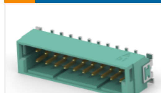
TE Part #464688-E DRCQ 2,54 20 M * SMD * 137 E012 167 GU-H
