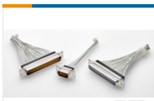
TE Part #2335890-5 AMPLIMITE SZ 5 RECEPT 50 POS, ST STL SHEL
