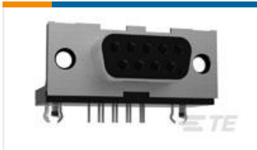
TE Part #3-106507-2 25P.HDP20 REC.ASSY.
