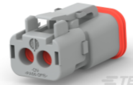
TE Part #1-2303815-2 DT06-2S-TN31, PLG, 2P, GRY, N, SNAPCAP
