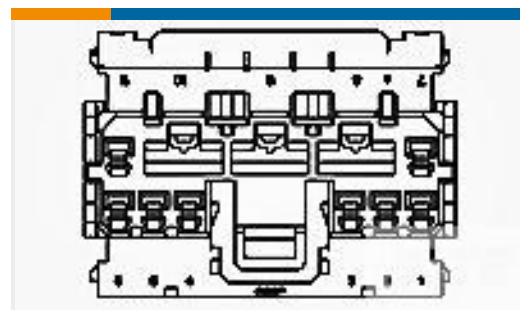
TE Part #85113-1 070/250 HYBRID 15P PLUG
