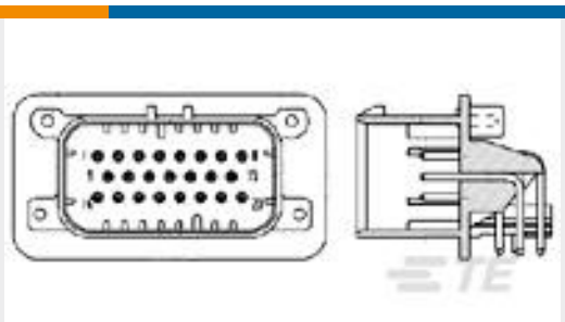
TE Part #1-776267-1 14POS,PIN DIA 1.3,HDR ASSY,90DEG, COD 1
