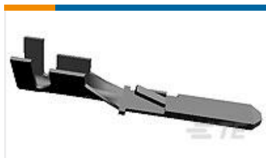
TE Part #160887-4 FF 110 TAB 0.5-1.0MM2 PTPPB
