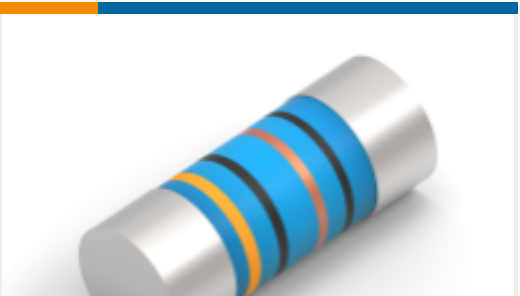
TE Part #1-2176315-1 MELF SMA_A 680R 0.1% 15PPM 0204 0.4W
