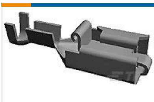
TE Part #170266-2 POSITIVE LOCK RECEPTACLE ELECTRO TPBR
