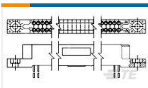
TE Part #531142-5 2 ROW BOX RECP 50 POS STAG
