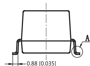
Right View
