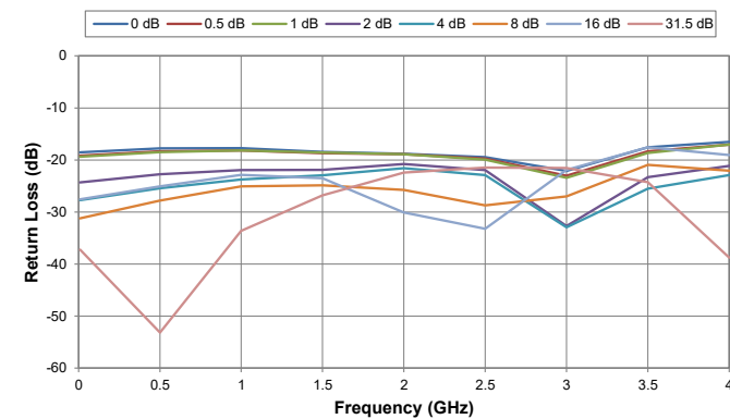
Figure 11. Output Return Loss vs Frequency @ Major
