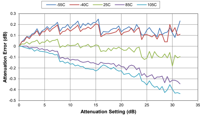
Figure 19. Attenuation Error @ 10 MHz vs
