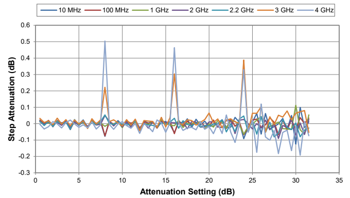
Figure 16. 0.5 dB Step Attenuation vs Attenuation
