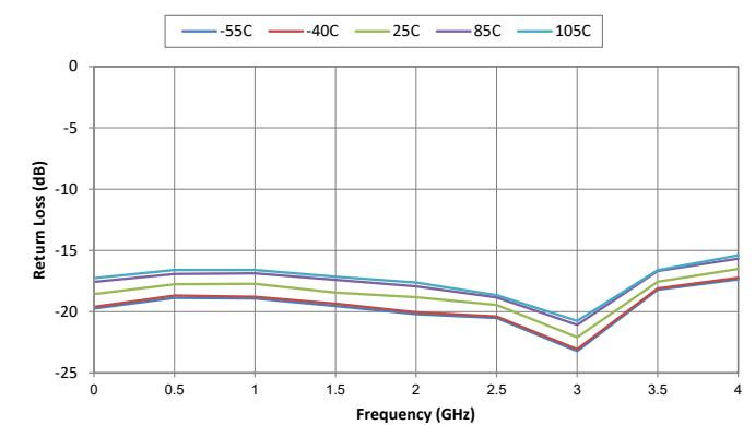
Figure 12. Output Return Loss vs Temperature
