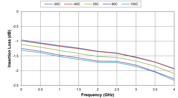
Figure 8. Insertion Loss vs Temperature
