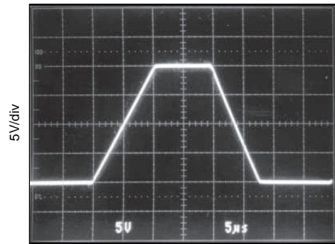
LARGE-SIGNAL STEP RESPONSE G = 1 , C_L = 100\text{pF}
