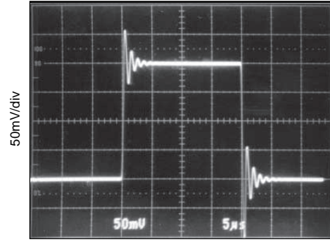
SMALL-SIGNAL STEP RESPONSE G = 1 , C_L = 1000\text{pF}
