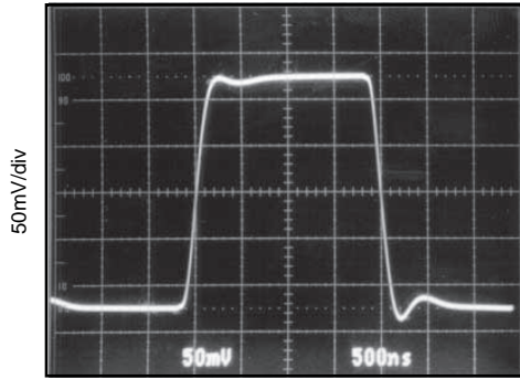
SMALL-SIGNAL STEP RESPONSE G = 1 , C_L = 100\text{pF}
