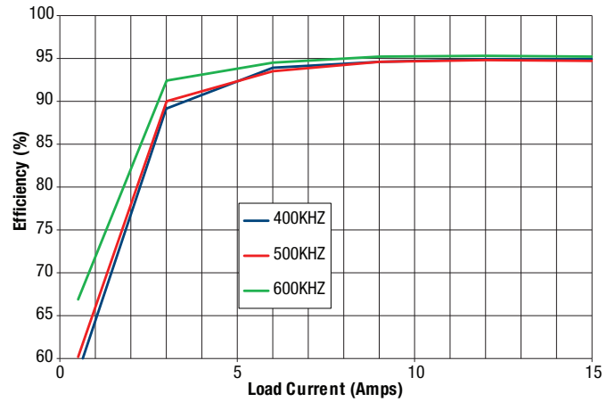
Efficiency vs. Load Current (Vo=3.3V, Vin=12Vin, 25°C, 100LFM)
