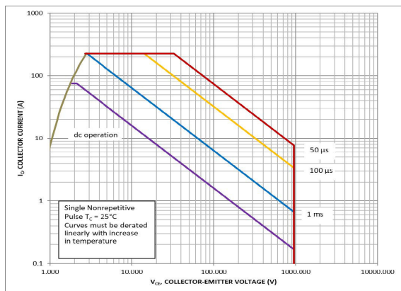
Figure 6. FBSOA
