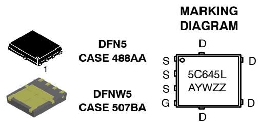
N-CHANNEL MOSFET
