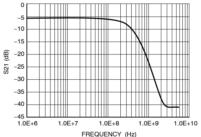
Figure 2. Insertion Loss Characteristic
