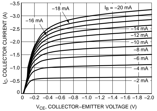
Figure 20. Output Characteristics
