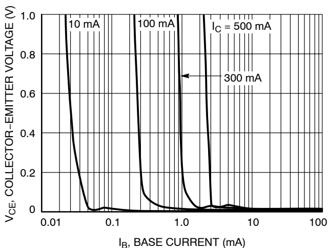
Figure 6. Saturation Region
