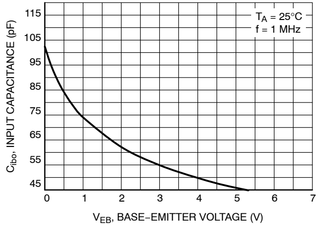
Figure 10. Input Capacitance
