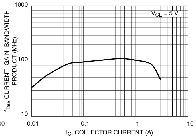
Figure 10. Current-Gain-Bandwidth Product
