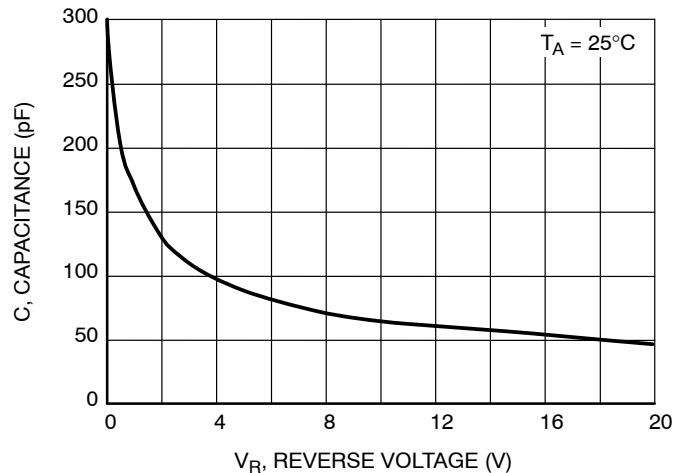
Figure 3. Typical Capacitance
