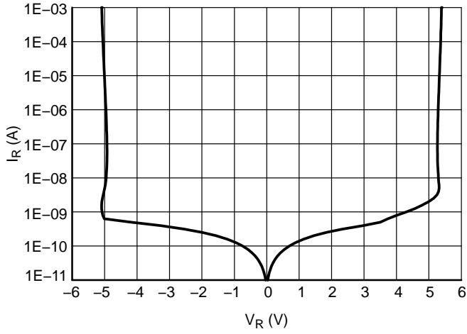
Figure 7. Breakdown Voltage
