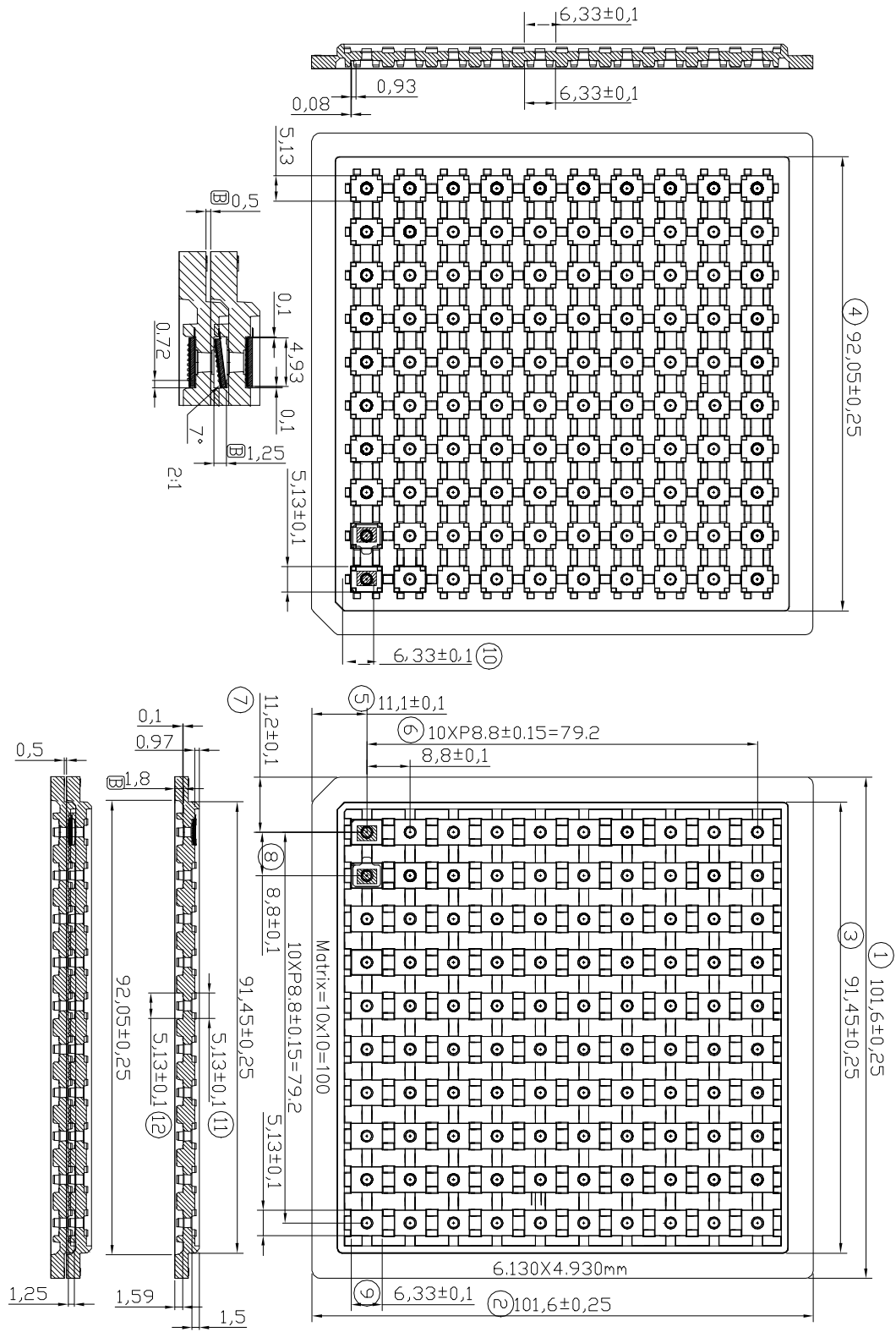
Figure 45. Tray Drawing
