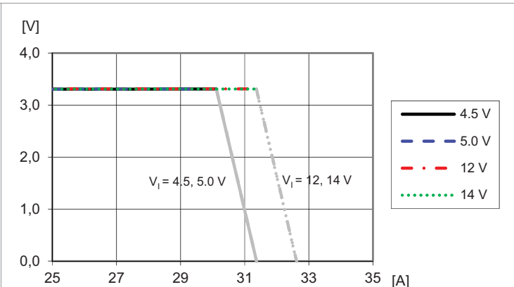
Current Limit Characteristics, V_O = 3.3 V
