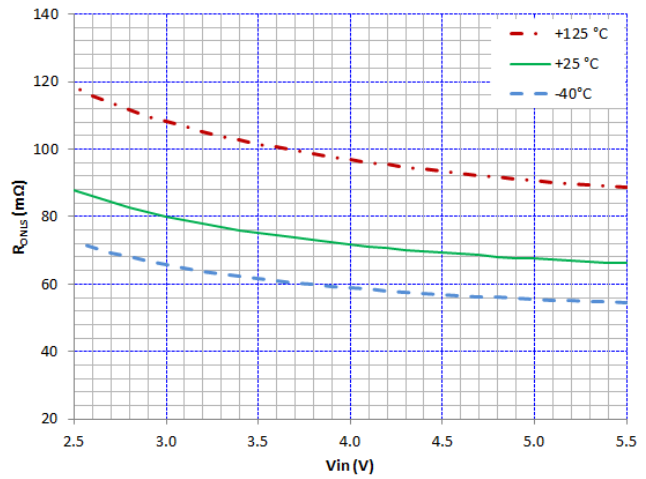
Figure 31. LSS R_{DS(on)} vs. V_{IN} and Temperature
