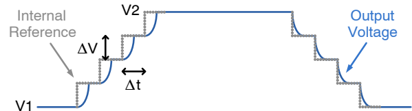
Figure 51. DVS in Forced PWM Mode Diagram
