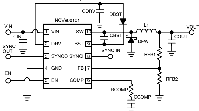
Figure 1. Typical Application
